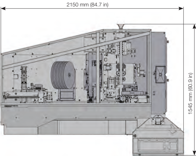
Machine height with closed safety cover 1765 mm (69.5 in.) Machine height with open safety cover 2765 mm (108.8 in.)
